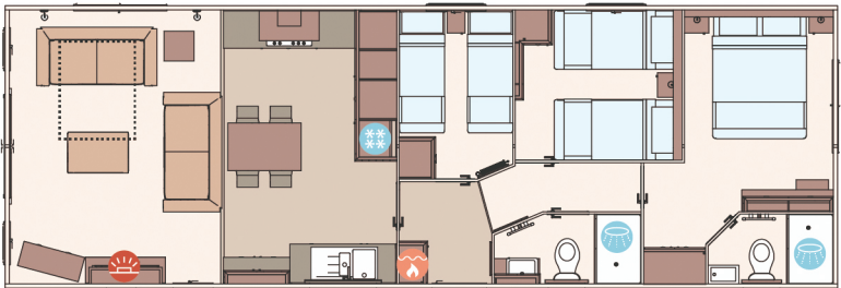
PREMIER 41FT X 14FT X 3 BEDROOM
