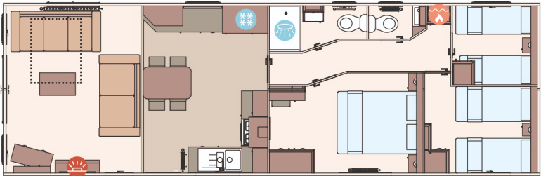
RESIDENTIAL 40FT X 13FT X 3 BEDROOM
